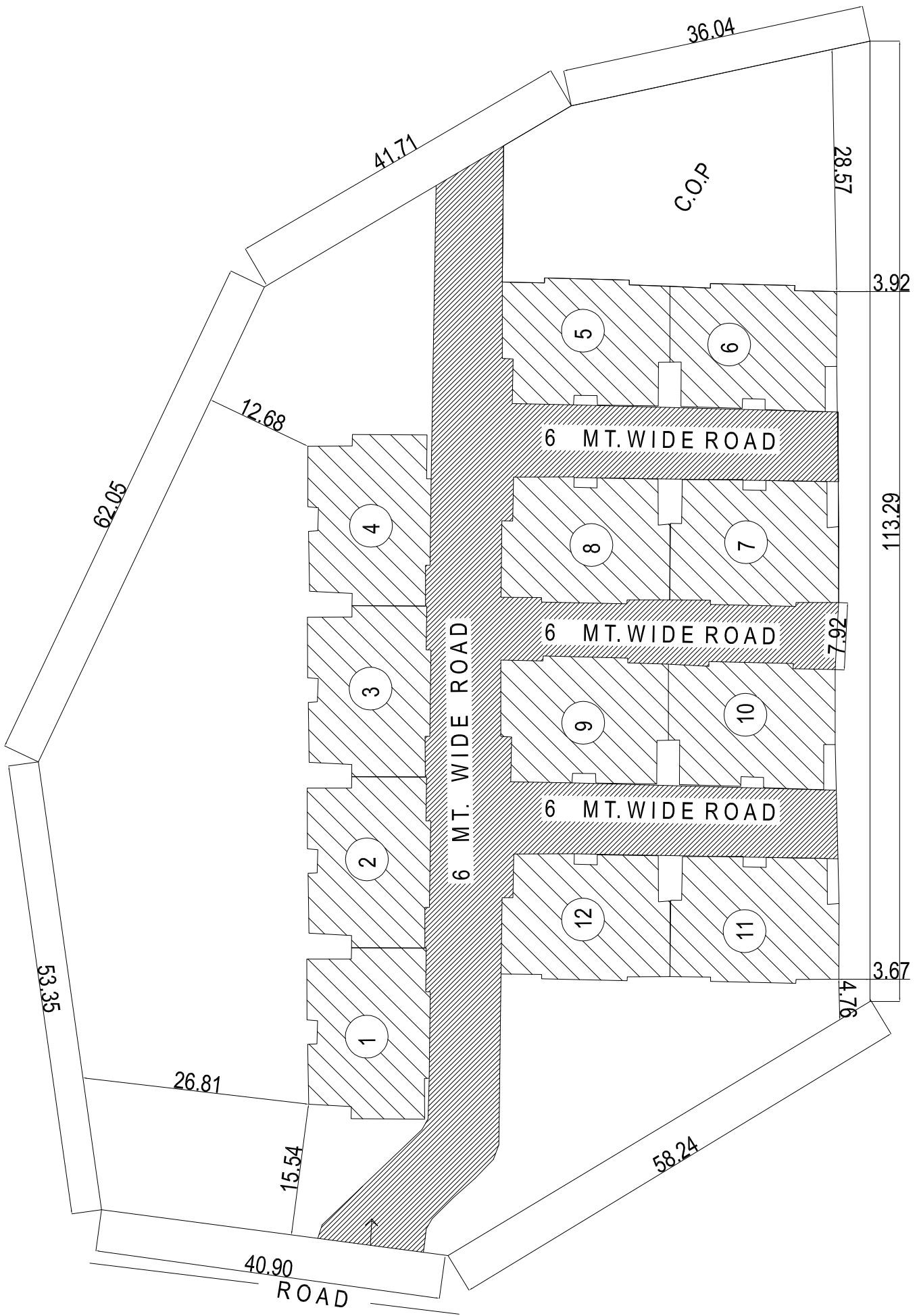
LAY-OUT OF T.P.NO-33,(DUMBHAL) F.P. NO.-R-21
